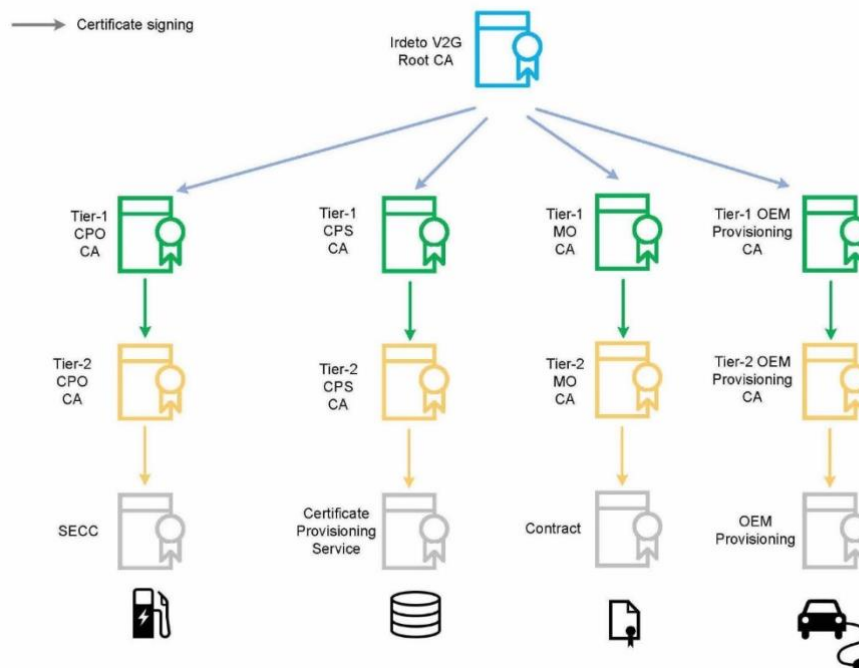
Figure 1: Overview of the Irdeto CrossCharge V2G PKI for ISO 15118-2
