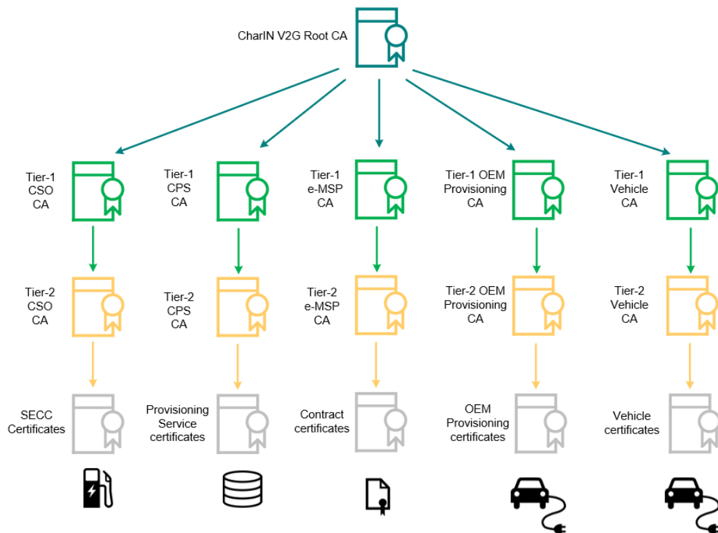
Figure 1: Overview of the CharIN V2G PKI for ISO 15118-20
